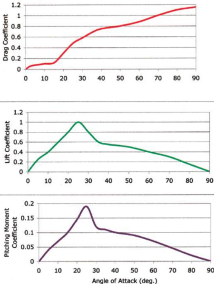
FIGURE 2. DEPENDENCE OF AERODYNAMIC COEFFICIENTS ON THE ANGLE OF ATTACK (ADAPTED FROM HUBBARD & CHENG, 2007).
