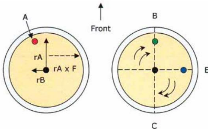
FIGURE 4. VIEW FROM TOP. EFFECT OF AIR ON THE CLOCKWISE ROTATING DISCUS CAUSING GYROSCOPIC PRECESSION ( rA \times F ), AND LATERAL DISPLACEMENT OF THE CENTER OF PRESSURE (A). IN THE RIGHT, A TORQUE ACTING ON POINT B (GREEN DOT), WILL CAUSE A PRECESSION OF THAT TORQUE 90° TOWARDS THE DIRECTION OF ROTATION CREATING A TORQUE VECTOR APPLYING A FORCE UPWARDS ON POINT E (BLUE DOT), CAUSING THE DISCUS TO ROTATE AROUND THE BC AXIS. (ADAPTED FROM BARTLETT, 1992).
